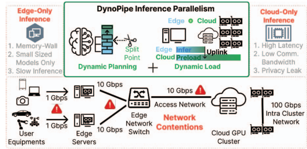
Fig. 1: DYNOPIPE addresses the fundamental trilemma of edge LLM deployment: computational bottlenecks at the edge, network latency in cloud offloading, and resource fragmentation across the edge-cloud continuum through adaptive pipeline parallelism with dynamic boundary shifting.
