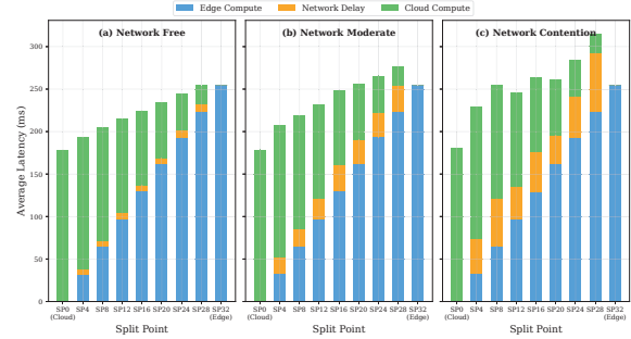
Fig. 15: Latency breakdown with heterogeneous edge GPU (30% slowdown). Edge computation penalty accumulates with more layers assigned to edge, making cloud-heavy split points more efficient for single requests while pipeline parallelism favors balanced splits under load.
