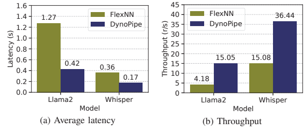
Fig. 16: Performance comparison of DYNOPipe and FlexNN in edge-only deployment. (a) Average latency reduction, (b) Throughput improvement.
